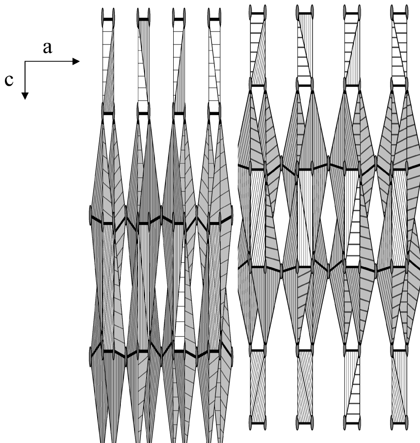
Figure 3 A polyhedral representation of the sodium titanium silicate structure showing structural features in the c -axis direction. The hexagonal cavities contain sodium ions which are omitted for clarity.
